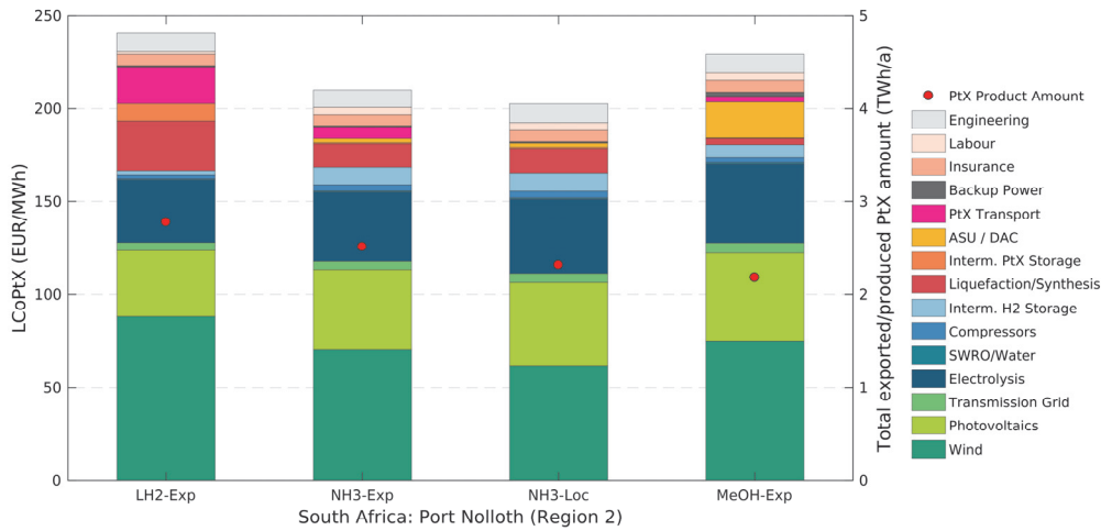
Figure 9-75: Cost breakdowns (left y-axis) and total PtX product amounts (right y-axis) for the South African site “Port Nolloth” (Region 2) and the assessed PtX energy carriers and their local production (-Loc) or supply cost (-Exp) including transport to Germany. The costs shown here apply to the respective cost-optimal system layout. The respective energy demands of individual components (such as electrolysis or compressors) are included in the cost shares of wind and PV (and not in the cost share of the electrolysis or compressors). The reason is that the systems are almost exclusively supplied by the local dedicated wind and PV plants. Therefore, the energy demand of a specific component directly affects the installed capacities of wind and PV.
