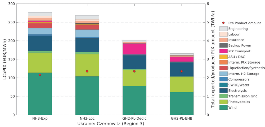
Figure 9-101: Cost breakdowns (left y-axis) and total PtX product amounts (right y-axis) for the Ukrainian site “Chernivtsi” (Region 3) and the assessed PtX energy carriers and their local production (-Loc) or supply cost (-Exp) including transport to Germany. The costs shown here apply to the respective cost-optimal system layout. The respective energy demands of individual components (such as electrolysis or compressors) are included in the cost shares of wind and PV (and not in the cost share of the electrolysis or compressors). The reason is that the systems are almost exclusively supplied by the local dedicated wind and PV plants. Therefore, the energy demand of a specific component directly affects the installed capacities of wind and PV.
