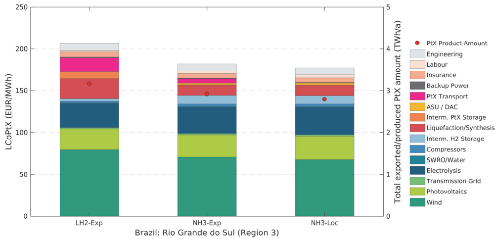
Figure 9-27: Cost breakdowns (left y-axis) and total PtX product amounts (right y-axis) for the Brazilian site “Rio Grande do Sul” (Region 3) and the assessed PtX energy carriers and their local production (-Loc) or supply cost (-Exp) including transport to Germany. The costs shown here apply to the respective cost-optimal system layout. The respective energy demands of individual components (such as electrolysis or compressors) are included in the cost shares of wind and PV (and not in the cost share of the electrolysis or compressors). The reason is that the systems are almost exclusively supplied by the local dedicated wind and PV plants. Therefore, the energy demand of a specific component directly affects the installed capacities of wind and PV.
