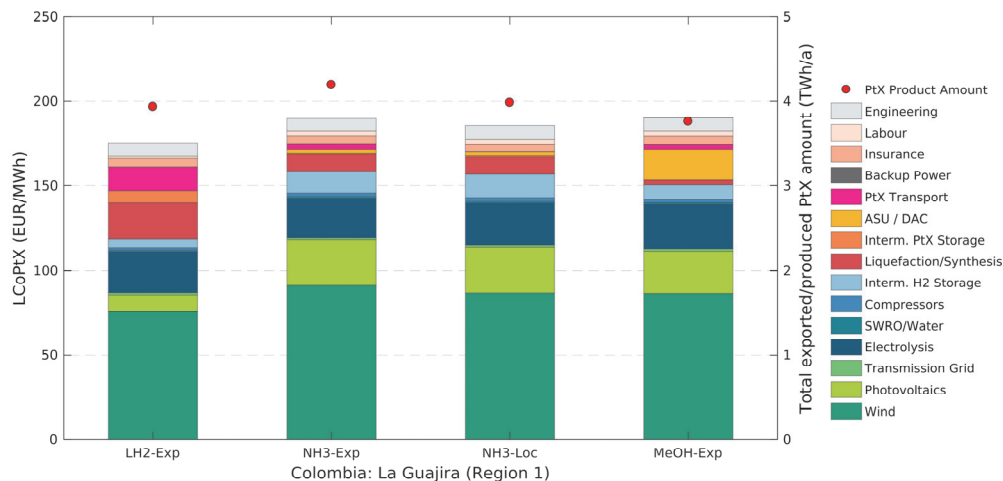
Figure 6-18: Cost breakdown and total PtX product amounts for the Colombian location Guajira/Uribea (Region 1) for four product scenarios exported liquid hydrogen (LH2-Exp), exported ammonia and methanol (NH3-Exp, MeOH-Exp) and the local distribution of ammonia (NH3-Loc). The costs shown here apply to the respective cost-optimal system layout.
