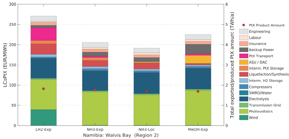
Figure 9-67: Cost breakdowns (left y-axis) and total PtX product amounts (right y-axis) for the Namibian site “Walvis Bay” (Region 2) and the assessed PtX energy carriers and their local production (-Loc) or supply cost (-Exp) including transport to Germany. The costs shown here apply to the respective cost-optimal system layout. The respective energy demands of individual components (such as electrolysis or compressors) are included in the cost shares of wind and PV (and not in the cost share of the electrolysis or compressors). The reason is that the systems are almost exclusively supplied by the local dedicated wind and PV plants. Therefore, the energy demand of a specific component directly affects the installed capacities of wind and PV.
