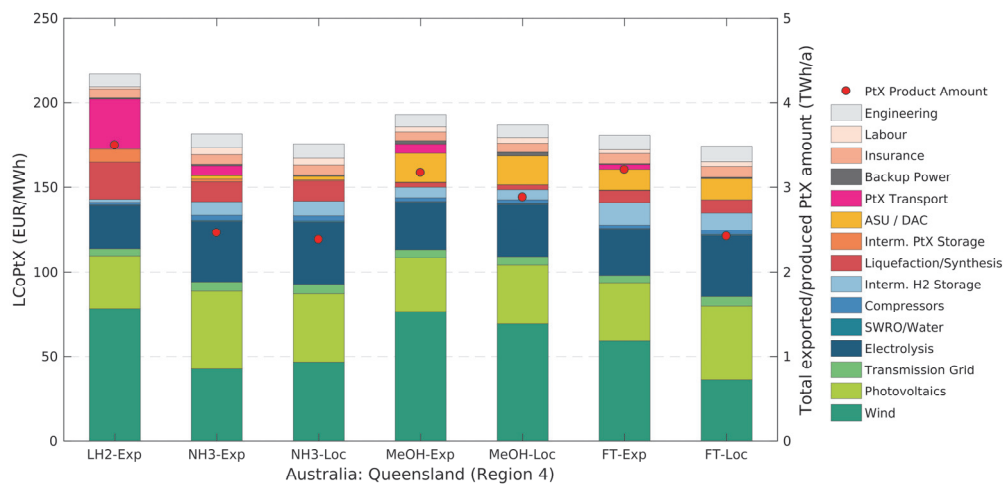
Figure 9-19: Cost breakdowns (left y-axis) and total PtX product amounts (right y-axis) for the Australian site “Queensland” (Region 4) and the assessed PtX energy carriers and their local production (-Loc) or supply cost (-Exp) including transport to Germany. The costs shown here apply to the respective cost-optimal system layout. The respective energy demands of individual components (such as electrolysis or compressors) are included in the cost shares of wind and PV (and not in the cost share of the electrolysis or compressors). The reason is that the systems are almost exclusively supplied by the local dedicated wind and PV plants. Therefore, the energy demand of a specific component directly affects the installed capacities of wind and PV.
