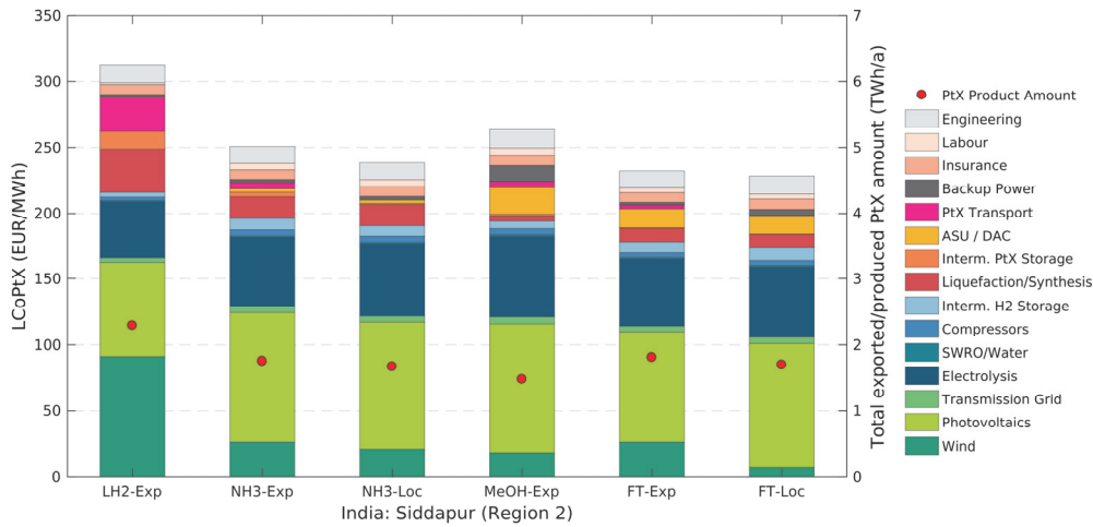
Figure 9-41: Cost breakdowns (left y-axis) and total PtX product amounts (right y-axis) for the Indian site “Siddapur” (Region 2) and the assessed PtX energy carriers and their local production (-Loc) or supply cost (-Exp) including transport to Germany. The costs shown here apply to the respective cost-optimal system layout. The respective energy demands of individual components (such as electrolysis or compressors) are included in the cost shares of wind and PV (and not in the cost share of the electrolysis or compressors). The reason is that the systems are almost exclusively supplied by the local dedicated wind and PV plants. Therefore, the energy demand of a specific component directly affects the installed capacities of wind and PV.
