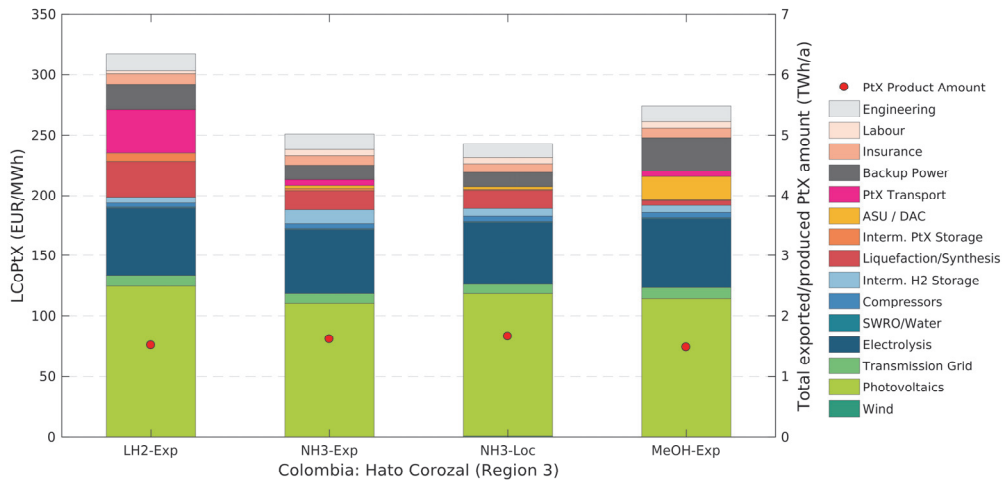
Figure 9-35: Cost breakdowns (left y-axis) and total PtX product amounts (right y-axis) for the Colombian site “Hato Corazol” (Region 3) and the assessed PtX energy carriers and their local production (-Loc) or supply cost (-Exp) including transport to Germany. The costs shown here apply to the respective cost-optimal system layout. The respective energy demands of individual components (such as electrolysis or compressors) are included in the cost shares of wind and PV (and not in the cost share of the electrolysis or compressors). The reason is that the systems are almost exclusively supplied by the local dedicated wind and PV plants. Therefore, the energy demand of a specific component directly affects the installed capacities of wind and PV.
