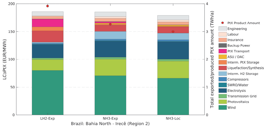
Figure 9-25: Cost breakdowns (left y-axis) and total PtX product amounts (right y-axis) for the Brazilian site “Bahia North – Irecê” (Region 2) and the assessed PtX energy carriers and their local production (-Loc) or supply cost (-Exp) including transport to Germany. The costs shown here apply to the respective cost-optimal system layout. The respective energy demands of individual components (such as electrolysis or compressors) are included in the cost shares of wind and PV (and not in the cost share of the electrolysis or compressors). The reason is that the systems are almost exclusively supplied by the local dedicated wind and PV plants. Therefore, the energy demand of a specific component directly affects the installed capacities of wind and PV.
