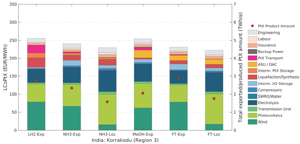
Figure 9-43: Cost breakdowns (left y-axis) and total PtX product amounts (right y-axis) for the Indian site “Korarakodu” (Region 3) and the assessed PtX energy carriers and their local production (-Loc) or supply cost (-Exp) including transport to Germany. The costs shown here apply to the respective cost-optimal system layout. The respective energy demands of individual components (such as electrolysis or compressors) are included in the cost shares of wind and PV (and not in the cost share of the electrolysis or compressors). The reason is that the systems are almost exclusively supplied by the local dedicated wind and PV plants. Therefore, the energy demand of a specific component directly affects the installed capacities of wind and PV.
