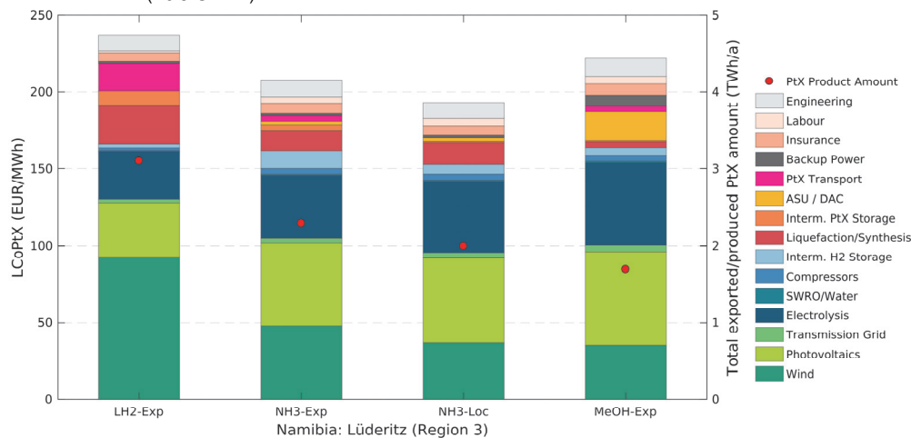
Figure 6-21: Cost breakdown and total PtX product amounts for the Namibian location Lüderitz (Region 3) for four product scenarios - exported liquid hydrogen (LH 2 -Exp), exported ammonia (NH 3 -Exp), local distribution of ammonia (NH 3 -Loc), and exported methanol based on DAC (MeOH-Exp). The costs shown here apply to the respective cost-optimal system layout.
