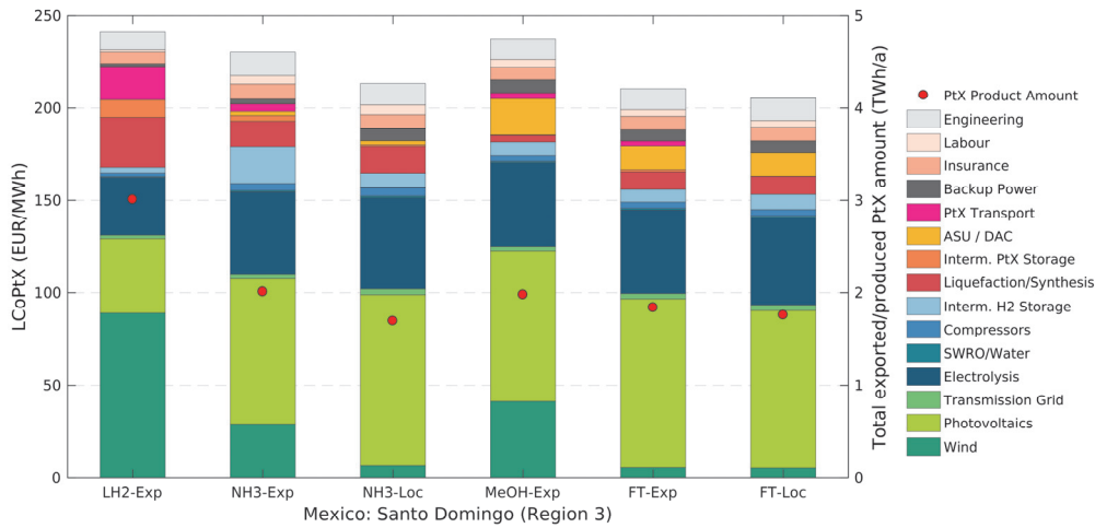
Figure 9-53: Cost breakdowns (left y-axis) and total PtX product amounts (right y-axis) for the Mexican site “Santo Domingo” (Region 3) and the assessed PtX energy carriers and their local production (-Loc) or supply cost (-Exp) including transport to Germany. The costs shown here apply to the respective cost-optimal system layout. The respective energy demands of individual components (such as electrolysis or compressors) are included in the cost shares of wind and PV (and not in the cost share of the electrolysis or compressors). The reason is that the systems are almost exclusively supplied by the local dedicated wind and PV plants. Therefore, the energy demand of a specific component directly affects the installed capacities of wind and PV.
