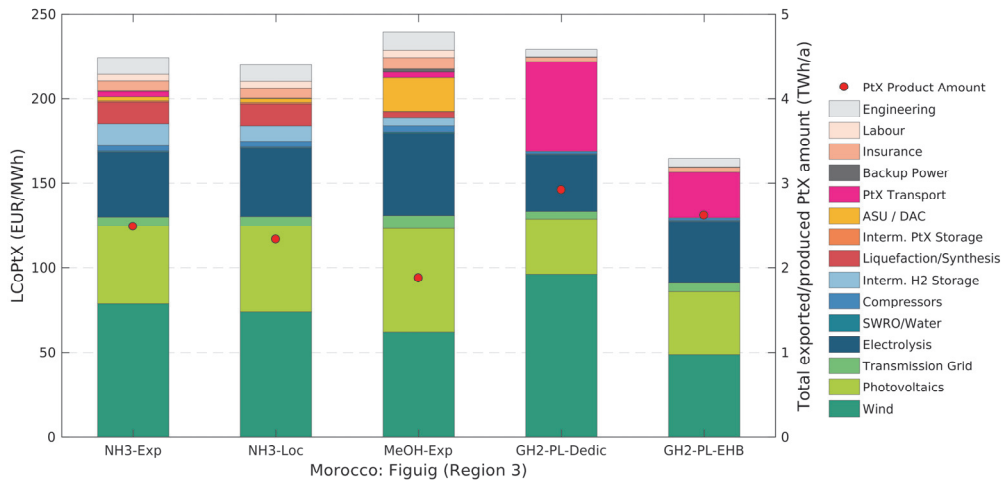
Figure 9-61: Cost breakdowns (left y-axis) and total PtX product amounts (right y-axis) for the Moroccan site “Figuiq” (Region 3) and the assessed PtX energy carriers and their local production (-Loc) or supply cost (-Exp) including transport to Germany. The costs shown here apply to the respective cost-optimal system layout. The respective energy demands of individual components (such as electrolysis or compressors) are included in the cost shares of wind and PV (and not in the cost share of the electrolysis or compressors). The reason is that the systems are almost exclusively supplied by the local dedicated wind and PV plants. Therefore, the energy demand of a specific component directly affects the installed capacities of wind and PV.
