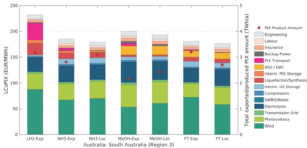
Figure 9-17: Cost breakdowns (left y-axis) and total PtX product amounts (right y-axis) for the Australian site “South Australia” (Region 3) and the assessed PtX energy carriers and their local production (-Loc) or supply cost (-Exp) including transport to Germany. The costs shown here apply to the respective cost-optimal system layout. The respective energy demands of individual components (such as electrolysis or compressors) are included in the cost shares of wind and PV (and not in the cost share of the electrolysis or compressors). The reason is that the systems are almost exclusively supplied by the local dedicated wind and PV plants. Therefore, the energy demand of a specific component directly affects the installed capacities of wind and PV.
