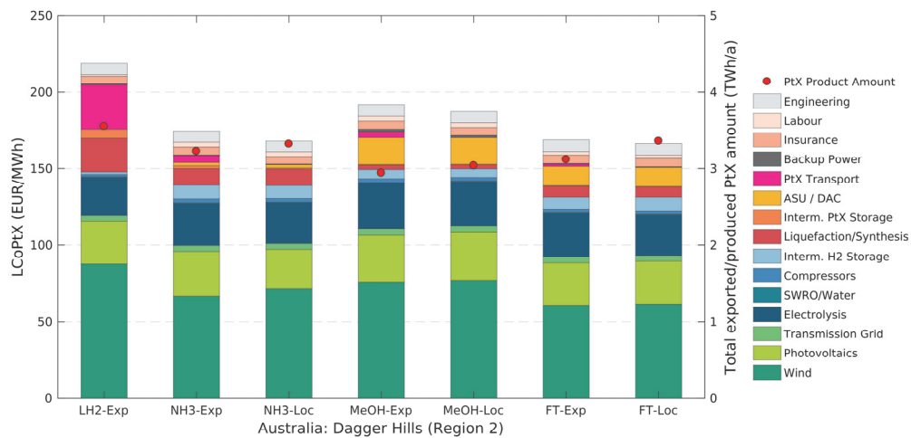
Figure 9-15: Cost breakdowns (left y-axis) and total PtX product amounts (right y-axis) for the Australian site “Dagger Hills” (Region 2) and the assessed PtX energy carriers and their local production (-Loc) or supply cost (-Exp) including transport to Germany. The costs shown here apply to the respective cost-optimal system layout. The respective energy demands of individual components (such as electrolysis or compressors) are included in the cost shares of wind and PV (and not in the cost share of the electrolysis or compressors). The reason is that the systems are almost exclusively supplied by the local dedicated wind and PV plants. Therefore, the energy demand of a specific component directly affects the installed capacities of wind and PV.
