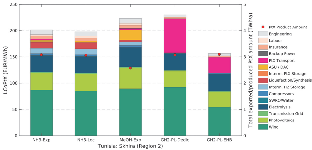
Figure 9-91: Cost breakdowns (left y-axis) and total PtX product amounts (right y-axis) for the Tunisian site “Shkira” (Region 2) and the assessed PtX energy carriers and their local production (-Loc) or supply cost (-Exp) including transport to Germany. The costs shown here apply to the respective cost-optimal system layout. The respective energy demands of individual components (such as electrolysis or compressors) are included in the cost shares of wind and PV (and not in the cost share of the electrolysis or compressors). The reason is that the systems are almost exclusively supplied by the local dedicated wind and PV plants. Therefore, the energy demand of a specific component directly affects the installed capacities of wind and PV.
