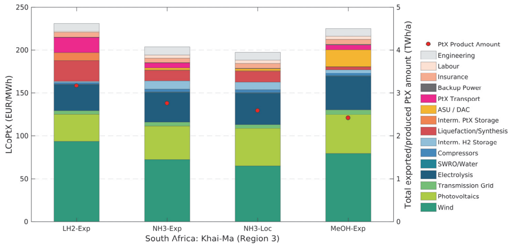
Figure 9-77: Cost breakdowns (left y-axis) and total PtX product amounts (right y-axis) for the South African site “Khai-Ma” (Region 3) and the assessed PtX energy carriers and their local production (-Loc) or supply cost (-Exp) including transport to Germany. The costs shown here apply to the respective cost-optimal system layout. The respective energy demands of individual components (such as electrolysis or compressors) are included in the cost shares of wind and PV (and not in the cost share of the electrolysis or compressors). The reason is that the systems are almost exclusively supplied by the local dedicated wind and PV plants. Therefore, the energy demand of a specific component directly affects the installed capacities of wind and PV.
