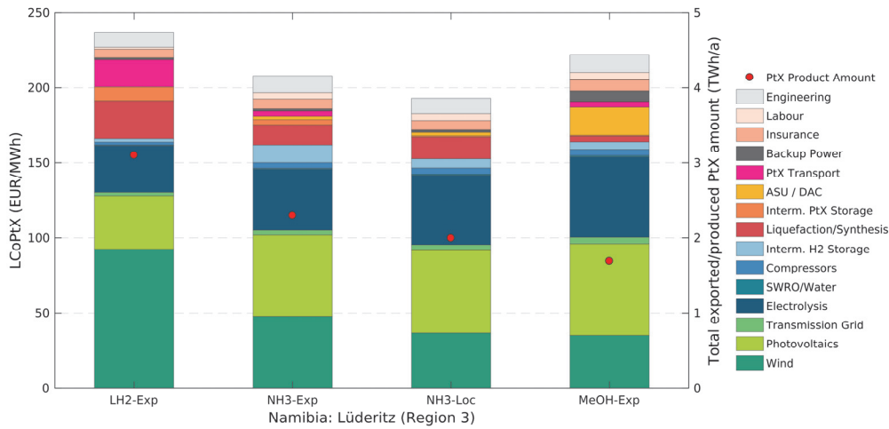
Figure 9-69: Cost breakdowns (left y-axis) and total PtX product amounts (right y-axis) for the Namibian site “Lüderitz” (Region 3) and the assessed PtX energy carriers and their local production (-Loc) or supply cost (-Exp) including transport to Germany. The costs shown here apply to the respective cost-optimal system layout. The respective energy demands of individual components (such as electrolysis or compressors) are included in the cost shares of wind and PV (and not in the cost share of the electrolysis or compressors). The reason is that the systems are almost exclusively supplied by the local dedicated wind and PV plants. Therefore, the energy demand of a specific component directly affects the installed capacities of wind and PV.
