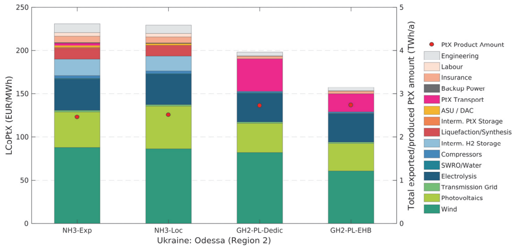
Figure 9-99: Cost breakdowns (left y-axis) and total PtX product amounts (right y-axis) for the Ukrainian site “Odessa” (Region 2) and the assessed PtX energy carriers and their local production (-Loc) or supply cost (-Exp) including transport to Germany. The costs shown here apply to the respective cost-optimal system layout. The respective energy demands of individual components (such as electrolysis or compressors) are included in the cost shares of wind and PV (and not in the cost share of the electrolysis or compressors). The reason is that the systems are almost exclusively supplied by the local dedicated wind and PV plants. Therefore, the energy demand of a specific component directly affects the installed capacities of wind and PV.
