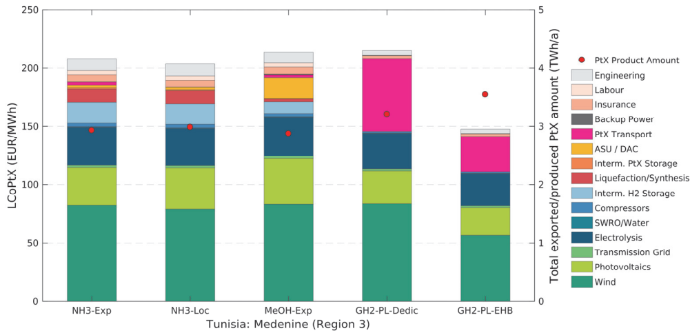
Figure 9-93: Cost breakdowns (left y-axis) and total PtX product amounts (right y-axis) for the Tunisian site “Medenine” (Region 3) and the assessed PtX energy carriers (–Loc) or supply cost (–Exp) including transport to Germany. The costs shown here apply to the respective cost-optimal system layout. The respective energy demands of individual components (such as electrolysis or compressors) are included in the cost shares of wind and PV (and not in the cost share of the electrolysis or compressors). The reason is that the systems are almost exclusively supplied by the local dedicated wind and PV plants. Therefore, the energy demand of a specific component directly affects the installed capacities of wind and PV.
