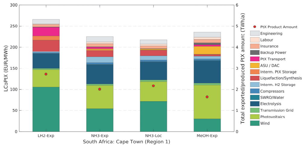
Figure 9-73: Cost breakdowns (left y-axis) and total PtX product amounts (right y-axis) for the South African site “Cape Town” (Region 1) and the assessed PtX energy carriers and their local production (-Loc) or supply cost (-Exp) including transport to Germany. The costs shown here apply to the respective cost-optimal system layout. The respective energy demands of individual components (such as electrolysis or compressors) are included in the cost shares of wind and PV (and not in the cost share of the electrolysis or compressors). The reason is that the systems are almost exclusively supplied by the local dedicated wind and PV plants. Therefore, the energy demand of a specific component directly affects the installed capacities of wind and PV.
