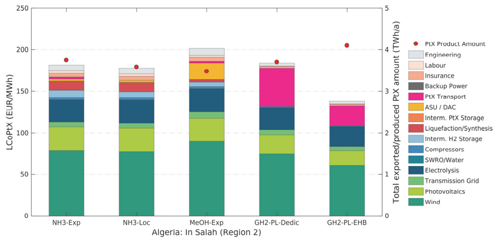
Figure 9-5: Cost breakdowns (left y-axis) and total PtX product amounts (right y-axis) for the Algerian site "In Salah" (Region 2) and the assessed PtX energy carriers and their local production (-Loc) or supply cost (-Exp) including transport to Germany. The costs shown here apply to the respective cost-optimal system layout. The respective energy demands of individual components (such as electrolysis or compressors) are included in the cost shares of wind and PV (and not in the cost share of the electrolysis or compressors). The reason is that the systems are almost exclusively supplied by the local dedicated wind and PV plants. Therefore, the energy demand of a specific component directly affects the installed capacities of wind and PV.
