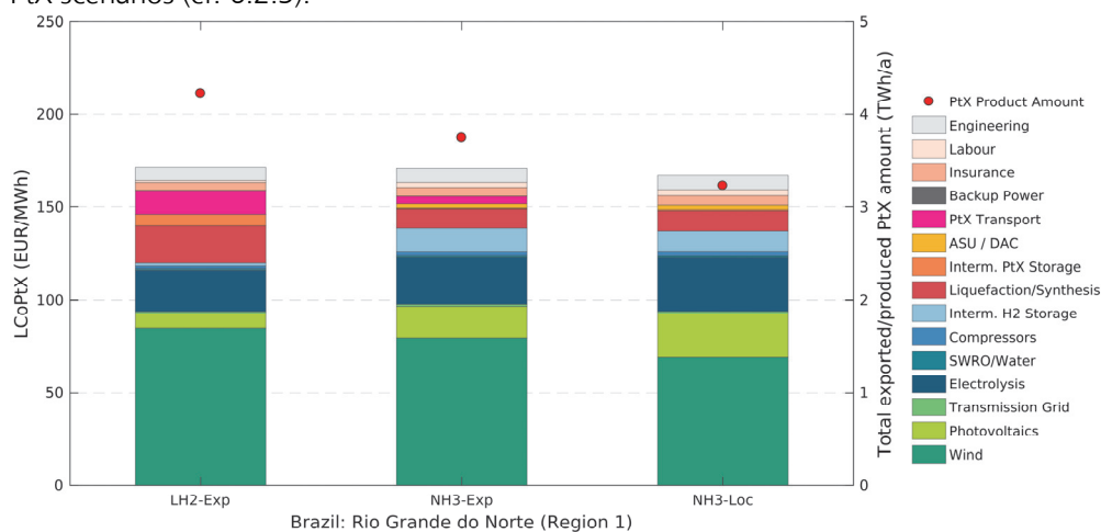
Figure 6-14: Cost breakdown and total PtX product amounts for the Brazilian location Rio Grande do Norte (Region 1) for three product scenarios – exported liquid hydrogen (LH2-Exp), exported and local distribution of ammonia (NH3-Exp, NH3-Loc, resp.). The costs shown here apply to the respective cost-optimal system layout.
