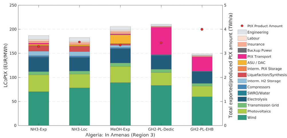
Figure 9-7: Cost breakdowns (left y-axis) and total PtX product amounts (right y-axis) for the Algerian site “In Amenas” (Region 3) and the assessed PtX energy carriers and their local production (-Loc) or supply cost (-Exp) including transport to Germany. The costs shown here apply to the respective cost-optimal system layout. The respective energy demands of individual components (such as electrolysis or compressors) are included in the cost shares of wind and PV (and not in the cost share of the electrolysis or compressors). The reason is that the systems are almost exclusively supplied by the local dedicated wind and PV plants. Therefore, the energy demand of a specific component directly affects the installed capacities of wind and PV.
