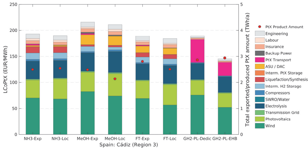
Figure 9-85: Cost breakdowns (left y-axis) and total PtX product amounts (right y-axis) for the Spanish site “Gibraltar/Cádiz” (Region 3) and the assessed PtX energy carriers and their local production (-Loc) or supply cost (-Exp) including transport to Germany. The costs shown here apply to the respective cost-optimal system layout. The respective energy demands of individual components (such as electrolysis or compressors) are included in the cost shares of wind and PV (and not in the cost share of the electrolysis or compressors). The reason is that the systems are almost exclusively supplied by the local dedicated wind and PV plants. Therefore, the energy demand of a specific component directly affects the installed capacities of wind and PV.
