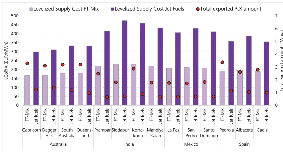
Figure 6-9: Jet fuel and Fischer-Tropsch product mix – levelized supply cost and total exported amount at the target port in Germany for all assessed locations and for PtX plants with an electrolysis capacity of 1 GW el . Cost include the capturing of atmospheric carbon dioxide with low-temperature DAC. A sensitivity analysis for the DAC CAPEX is included in section 6.3.1.
