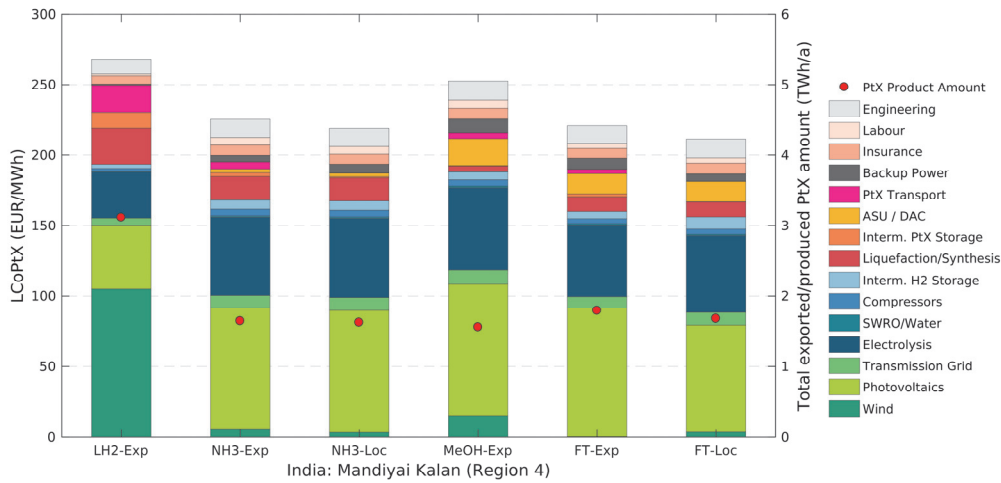
Figure 9-45: Cost breakdowns (left y-axis) and total PtX product amounts (right y-axis) for the Indian site “Mandiyai Kalan” (Region 4) and the assessed PtX energy carriers and their local production (-Loc) or supply cost (-Exp) including transport to Germany. The costs shown here apply to the respective cost-optimal system layout. The respective energy demands of individual components (such as electrolysis or compressors) are included in the cost shares of wind and PV (and not in the cost share of the electrolysis or compressors). The reason is that the systems are almost exclusively supplied by the local dedicated wind and PV plants. Therefore, the energy demand of a specific component directly affects the installed capacities of wind and PV.
