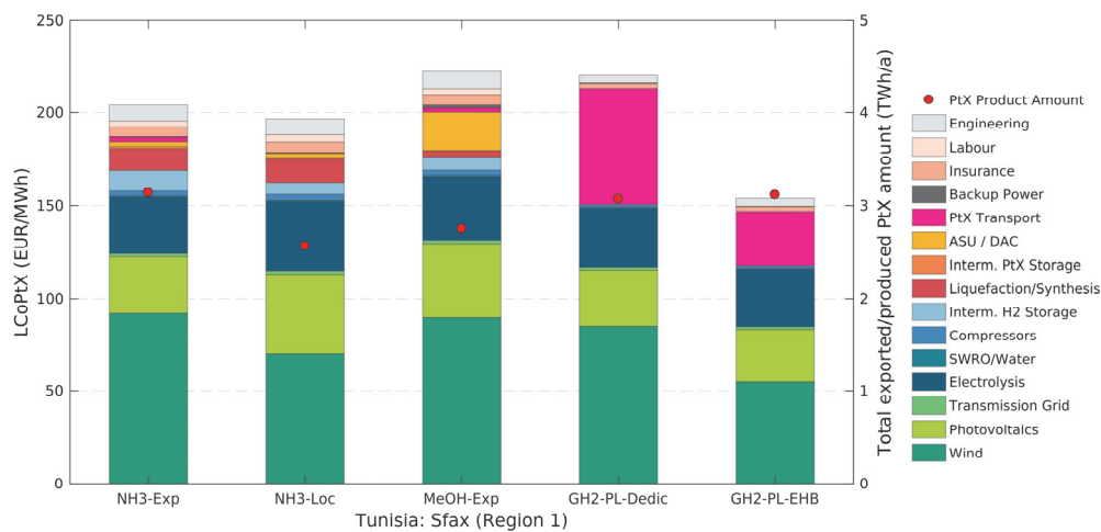
Figure 9-89: Cost breakdowns (left y-axis) and total PtX product amounts (right y-axis) for the Tunisian site “Sfax” (Region 1) and the assessed PtX energy carriers and their local production (-Loc) or supply cost (-Exp) including transport to Germany. The costs shown here apply to the respective cost-optimal system layout. The respective energy demands of individual components (such as electrolysis or compressors) are included in the cost shares of wind and PV (and not in the cost share of the electrolysis or compressors). The reason is that the systems are almost exclusively supplied by the local dedicated wind and PV plants. Therefore, the energy demand of a specific component directly affects the installed capacities of wind and PV.
